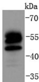
Fig. 1. Western blot analysis of FOXO4 on human lung lysates using anti-FOXO4 antibody at 1/1,000 dilution.
