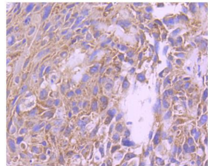
Fig. 2. Immunohistochemical analysis of paraffin-embedded human breast carcinoma tissue using anti-FOXO4 antibody. Counter stained with hematoxylin.
